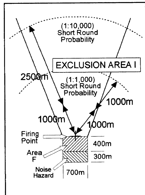
Figure J-3. Noise hazard area.
