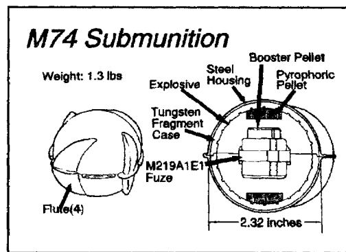
Figure 1-7. M74 submunition.
